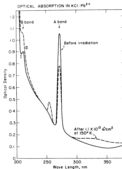
FIG. 2. Absorption spectra of KCl: \text{Pb}^{2+} in the near ultraviolet. Curve I: after quenching from 475^\circ\text{K} ; curve II: after exposure to 1.1 \times 10^{13} 1.5-MeV e^-/\text{cm}^2 at 150^\circ\text{K} . (All spectra measured at 80^\circ\text{K} .)
