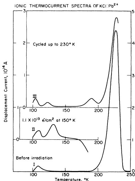
FIG. 1. Ionic thermocurrent spectra for KCl:Pb 2+ . Curve I: after quenching from 475°K; curve II: after exposure to 1.1 \times 10^{13} 1.5-MeV e^-/\text{cm}^2 at 150°K; curve III: after thermal cycling up to 230°K.
